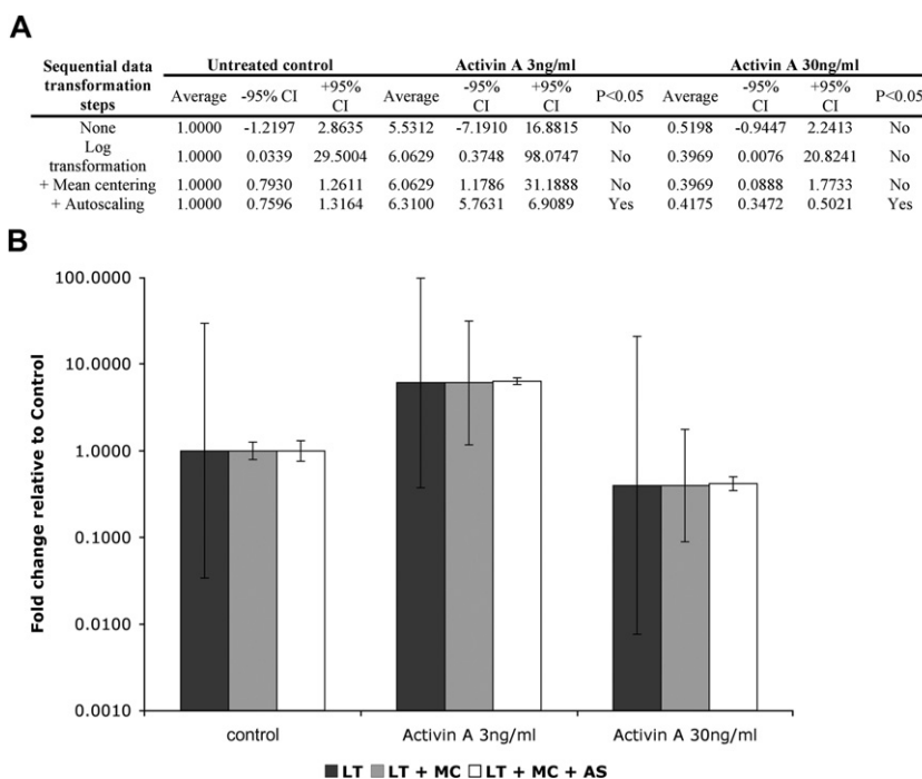
Fig. 2. Effect of sequential standardization steps on the statistical significance of Brachyury expression by Activin A in biological repeats. The effect of the sequential standardization steps on the average and the 95% CI (–95% CI, lower interval, and +95% CI, upper interval) is demonstrated in the table (A) as well as in the figure (B), representing the average (histograms) and 95% CI (error bars) after the sequential standardization steps (B). P < 0.05 indicates the significance of Brachyury induction or reduction by the Activin A treatment compared with untreated controls. LT, log transformation; MC, mean centering; AS, autoscaling.
